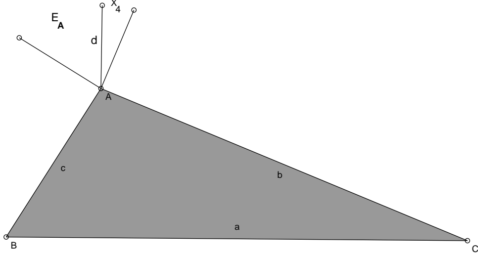
FIGURE 4. The case of an obtuse triangle and P = X_4
