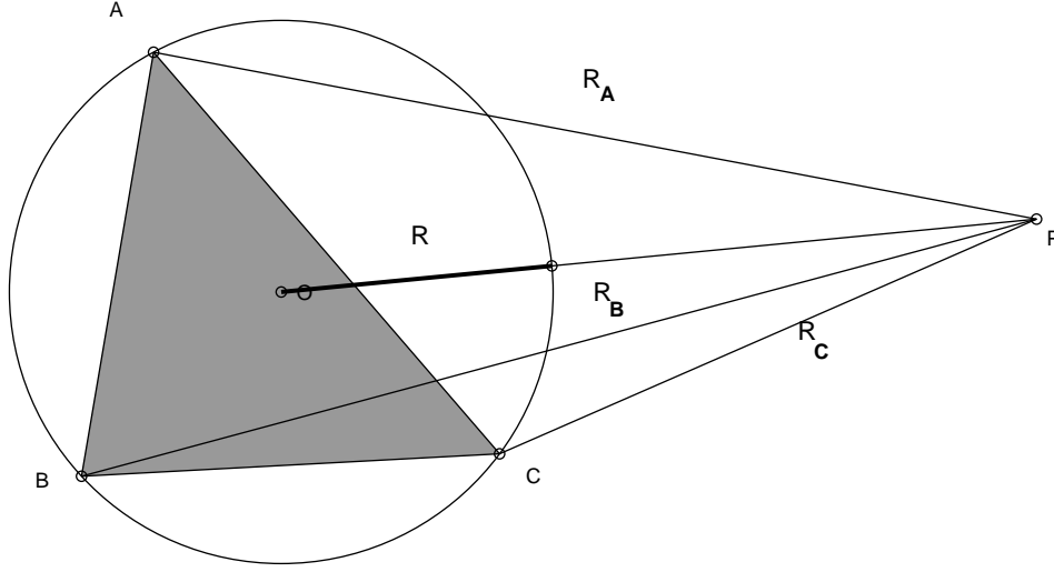
FIGURE 5. P is far from Int(ABC)
