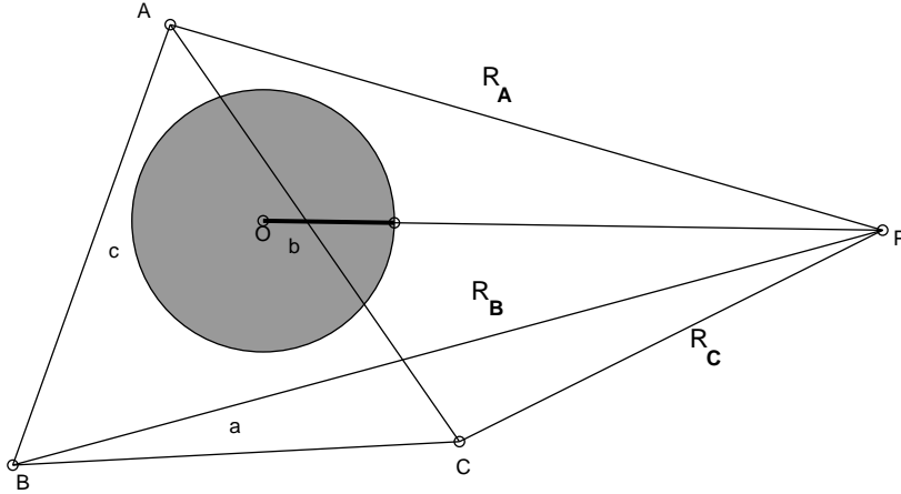
FIGURE 7. The case in that M is a disk
