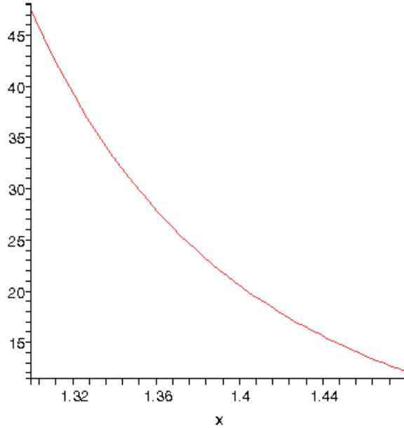
FIGURE 1. The plot for \zeta''(x)\zeta(x) - 2[\zeta'(x)]^2 on (1, \zeta^{-1}(e))
